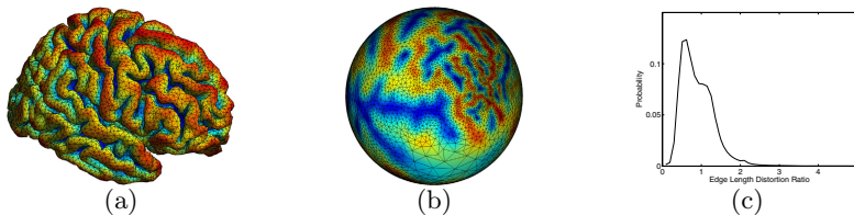
Fig. 1. Spherical conformal parameterization. (a) Cortical surface. (b) Projection of the cortical surface mesh onto the sphere with the conformal map to the sphere. (c) After surface area normalization, the distribution of the ratio of the length of corresponding edges in the mesh of (b) and (a).
