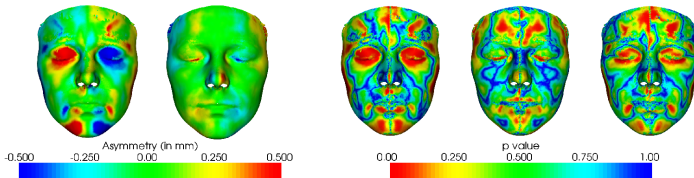
Fig. 4. Statistical analysis of asymmetry. Left to right: mean signed asymmetry maps on men/women, uncorrected p-value maps (using t -tests) of statistically significant asymmetry among men, among women, and comparison between men and women.
