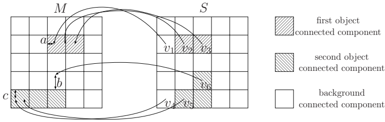
Fig. 1. Illustration of the computation of \rho(v, S, M, h) for 6 pixels. M is composed of two OCCs and of one BCC. \rho(v, S, M, h) is equal to 0 for v_2, v_3, and v_5 since h(v_2), h(v_3), and h(v_5) belong to the same CC as v_2, v_3, and v_5, respectively. However, v_6 belongs to the second OCC whereas h(v_6) belongs to the BCC so that \rho(v_6, S, M, h) is equal to b, namely, the distance between h(v_6) and the second OCC (in M ). In the same way, \rho(v_1, S, M, h) = a and \rho(v_4, S, M, h) = c.
