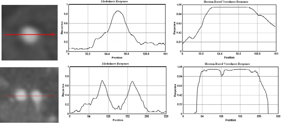
Fig. 1. This figure illustrates the medialness responses along a ray on two different examples obtained from our method (middle column) and the Hessian-based method (right column). Observe that unlike Hessian based methods, our technique gives low responses between two nearby vessels.
