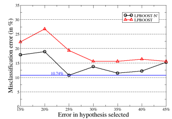
Fig. 3. Misclassification error for boosting on coordinates for LPBoost and LPBoost- N'
