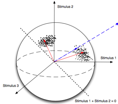
Fig. 1. An artificial population of voxels illustrating the space of activation profiles. The experiment presents three stimuli and evokes two distinct profiles. The blue, dashed line shows an original vector of regression coefficients. A hypothesis test comparing the first and second stimuli projects the vector of regression coefficients onto the dotted line; the significance is a function of the projection coefficient. The red vectors are the cluster mean profiles.
