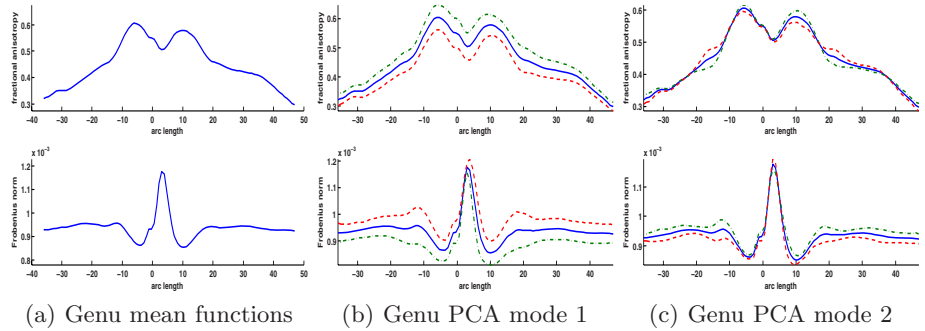
Fig. 3. Visualization of the PCA modes for the joint analysis of FA and Frobenius norm in the genu tract. The (a) mean functions for the combined population are shown with (b) the first and (c) second PCA modes. The first PCA mode accounts for a large percentage of the variability and shows an overall constant change in FA and an anti-correlated constant change in norm.
