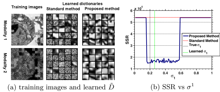
Fig. 3. \tilde{D} is learned from training SEM/confocal images with Gaussian noise (left). The curve (right) shows the robustness with respect to \sigma_1 . The vertical green dashed line indicates the learned \sigma_1 .
