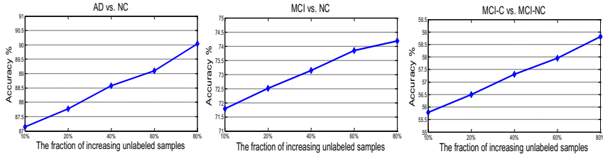
Fig. 1. Classification accuracy with different number of unlabeled samples
