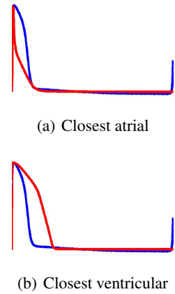
Fig. 3. Misclassified embryonic atrial AP (blue) and closest mature model APs (red)
