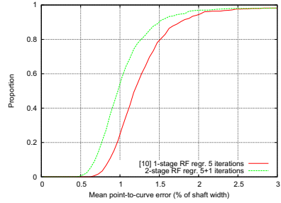
Fig. 4. Effect of introducing a second searching stage to locally refine point placements. Every Random Forest (RF) uses 10 trees
