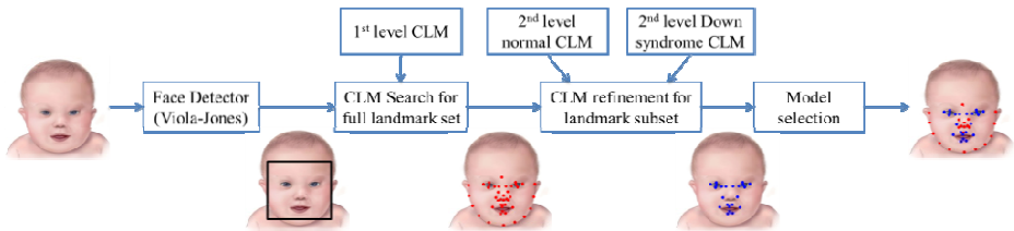
Fig. 1. The framework of hierarchical constrained local model (HCLM)
