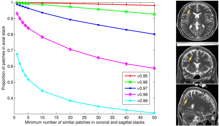
Fig. 1. Left: Quantitative check of self-similarity in a T2-weighted brain MRI from BrainWeb [12]. Similarity between the 10% axial 7x7 patches with the highest variance and all coronal and sagittal 7x7 patches was evaluated. For several similarity thresholds, the fraction of axial patches is plotted as function of the number of coronal and sagittal patches exceeding the threshold. Similarity is measured as the inner product between the patches (after vectorization and unit length normalization). Right: Example of local self-similarity in the cortex. The yellow arrows point at a similar cortex structure in the axial (top), coronal (middle), and sagittal (bottom) slices.
