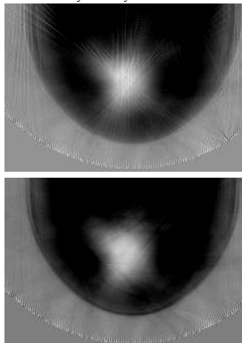
Figure 6. Top: Sound speed image of a simple phantom reconstructed from a numerical simulation using 256 array elements. Note the linear artifacts resulting from under- sampling. Bottom: Reconstruction of the same phantom using a simulation with 512 array elements. Note the suppression of the linear artifacts from just a modest improvement of the spacing interval.
